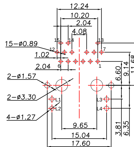
Suggested PCB Layout(Top View) (Tolerance:±0.05)
