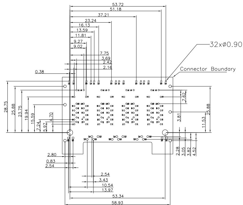
PCB Layout
