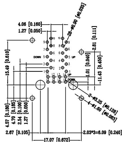
Suggested PCB Layout(Top View) (Tolerance:±0.05)
