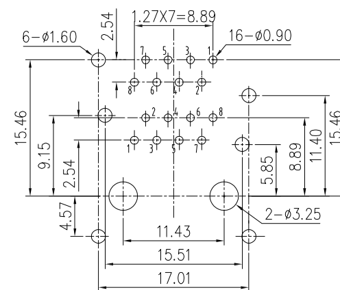
PC BOARD LAYOUT COMPONENT SIDE SHOWN THICKNESS=1.6mm
