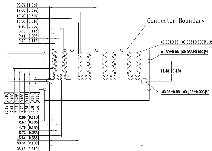
PCB Layout
